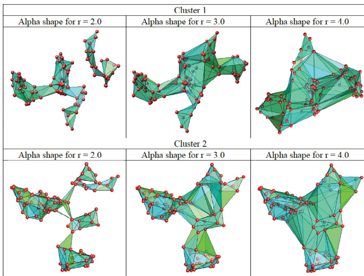
Figure 3: Representative alpha shapes for 2 clusters of the hierarchical analysis of conformers. For rolling ball of radius = 2.0 Å, 3.0Å and 4.0Å.
