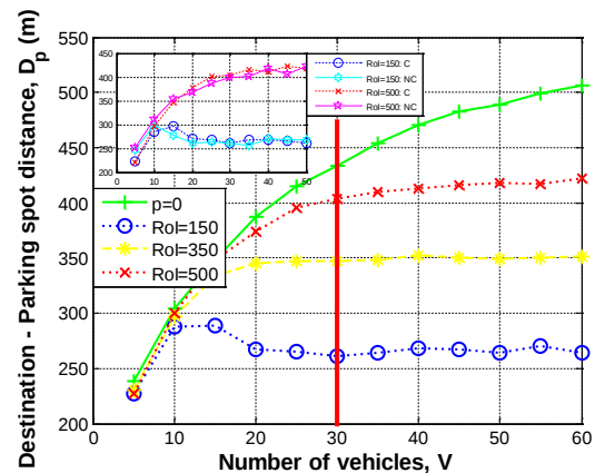
Σχήμα 20: Average destination-spot distance
