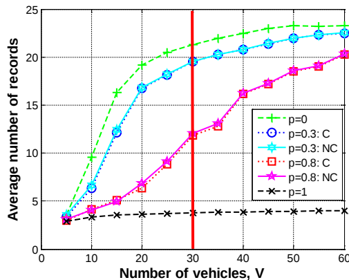
Σχήμα 13: Average number of records in memory
