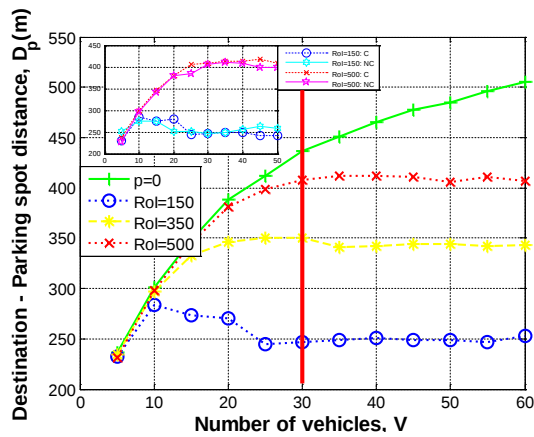
Σχήμα 6: Average destination-spot distance
